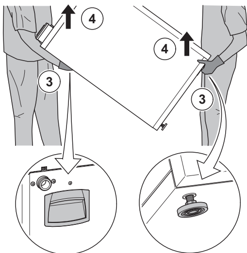
Abb.12 Manueller Transport
